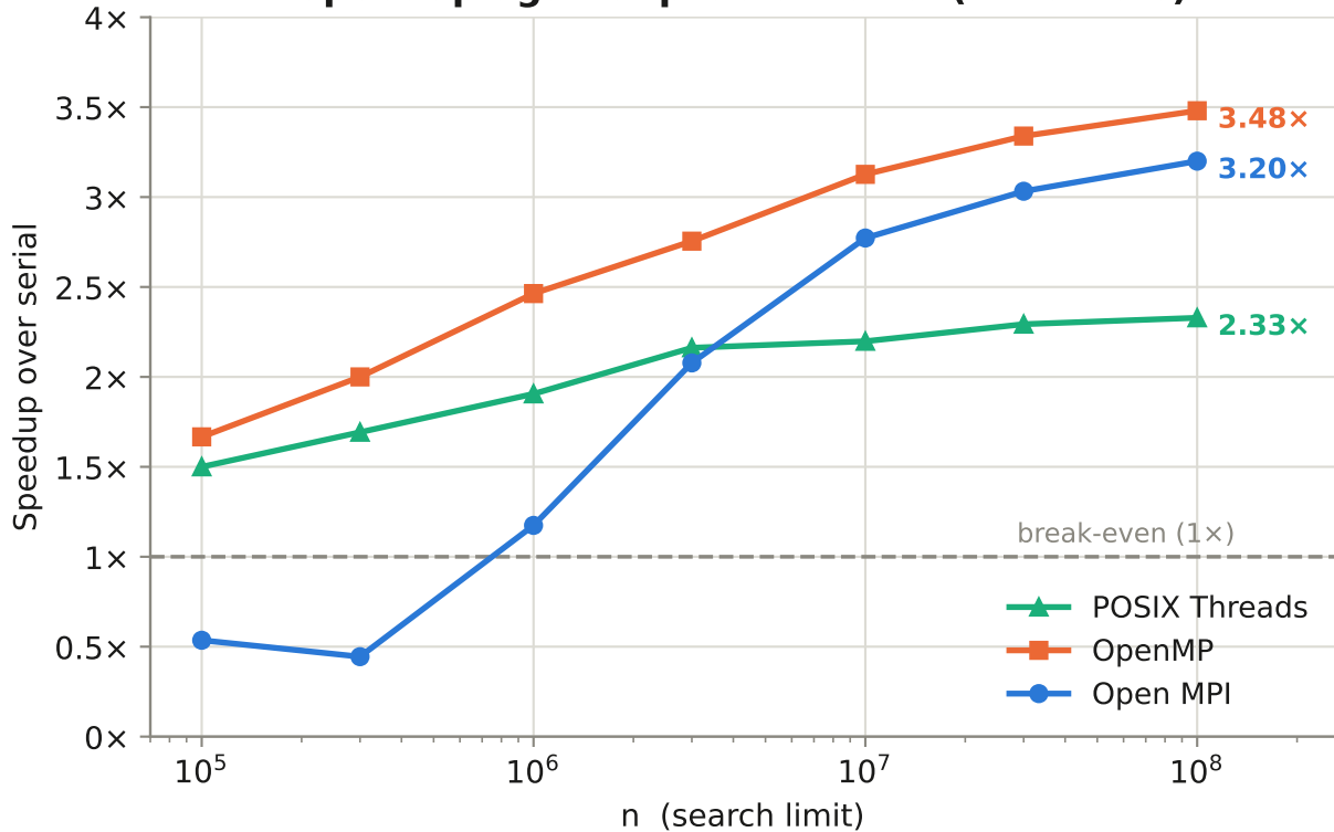
Speedup against problem size (4 workers)
